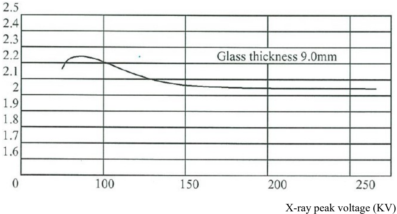
Fig. 2: Lead equivalent and X-ray peak voltage
